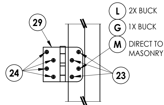
HINGE DETAIL
