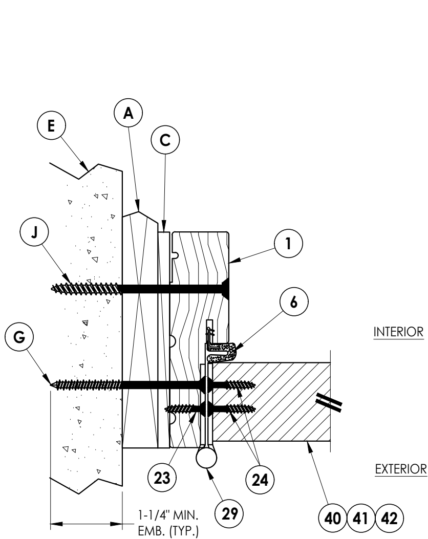
2 HORIZONTAL CROSS SECTION 6 Shown w/ 1X sub-buck Outswing shown (Inswing similar)
